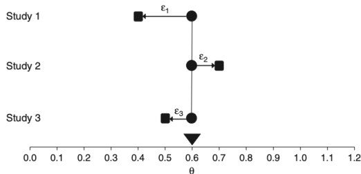
Figure: Fixed-effect model: distribution of sampling error
