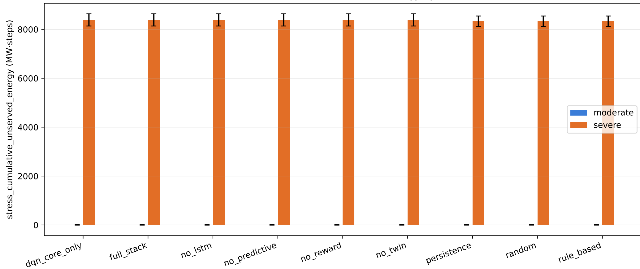
Stress-scenario cumulative unserved energy by controller
