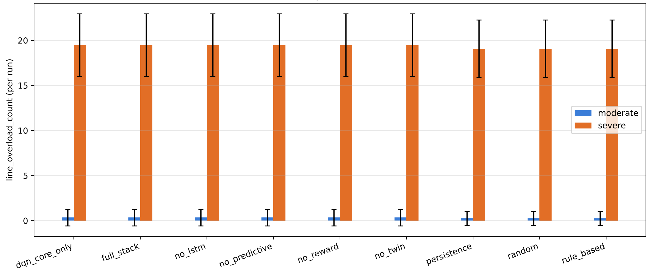
Line overload count by controller (stress benchmark)
