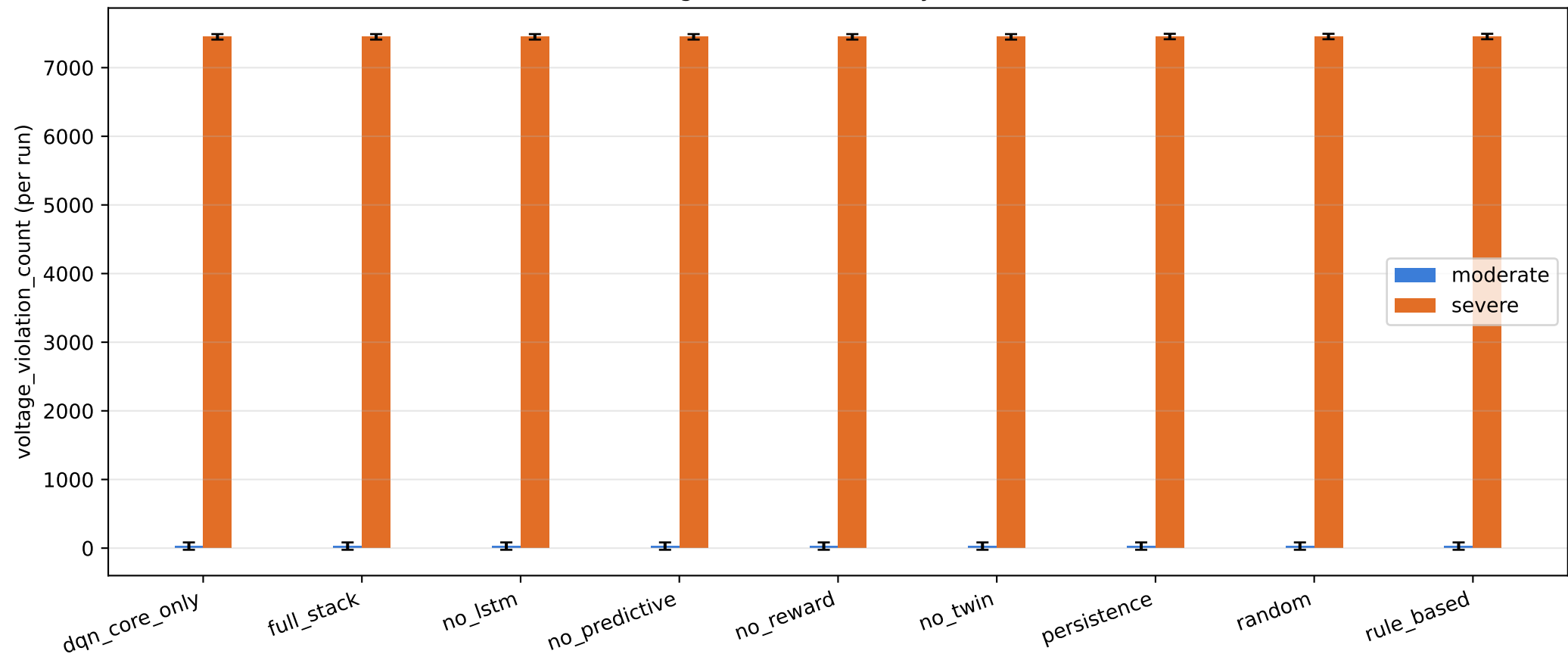
Voltage violation count by controller
