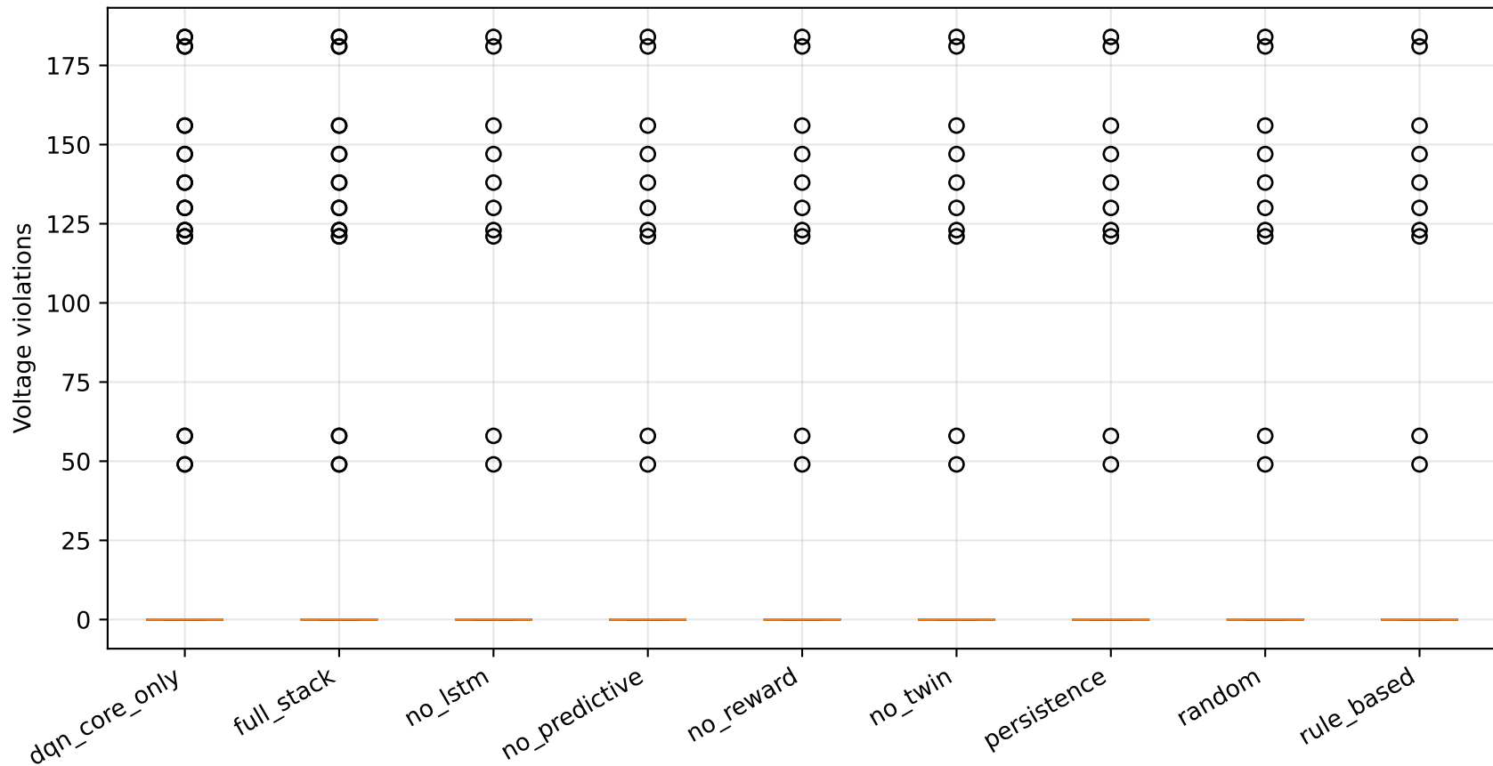
Voltage violation count by controller
