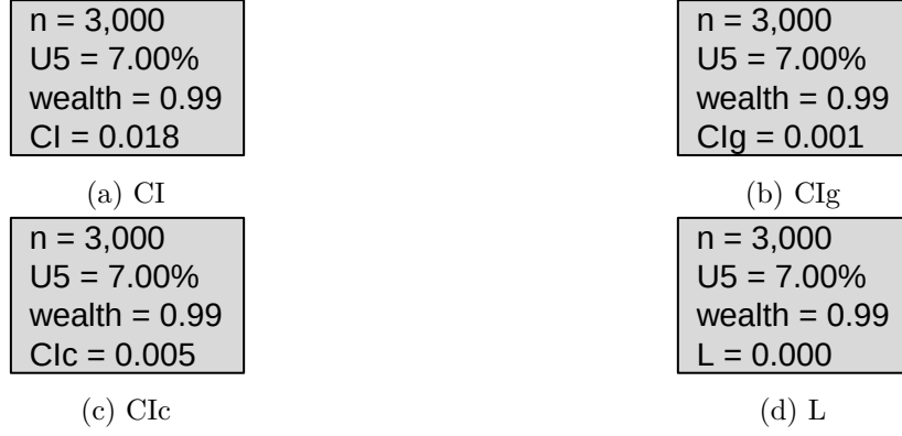
Figure 12: Null simulation concentration-index trees by criterion.
