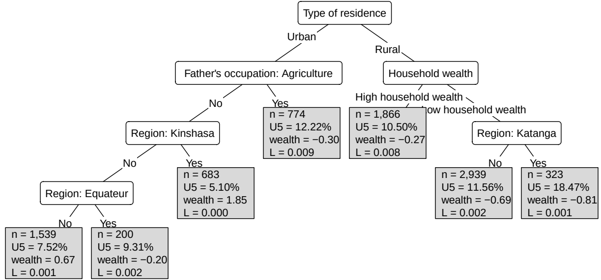
Figure 5: Level dependent concentration-index tree for under-five mortality in the DRC.
