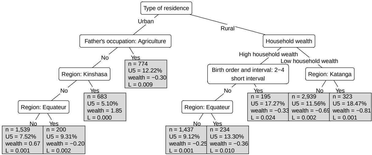
Figure 5: Level dependent concentration-index tree for under-five mortality in the DRC.
