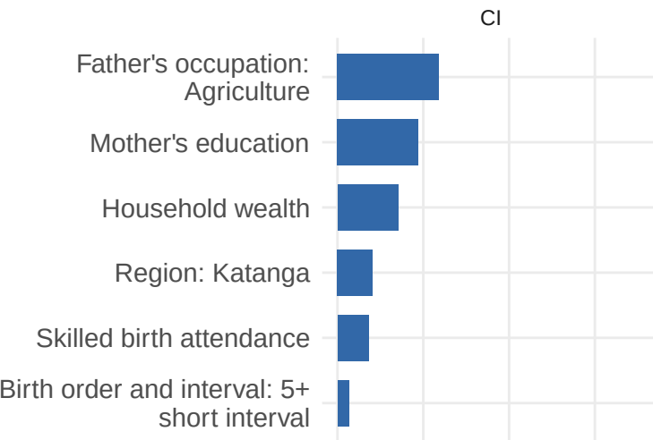
Top Tree Variables by Concentration-Index Criterion
