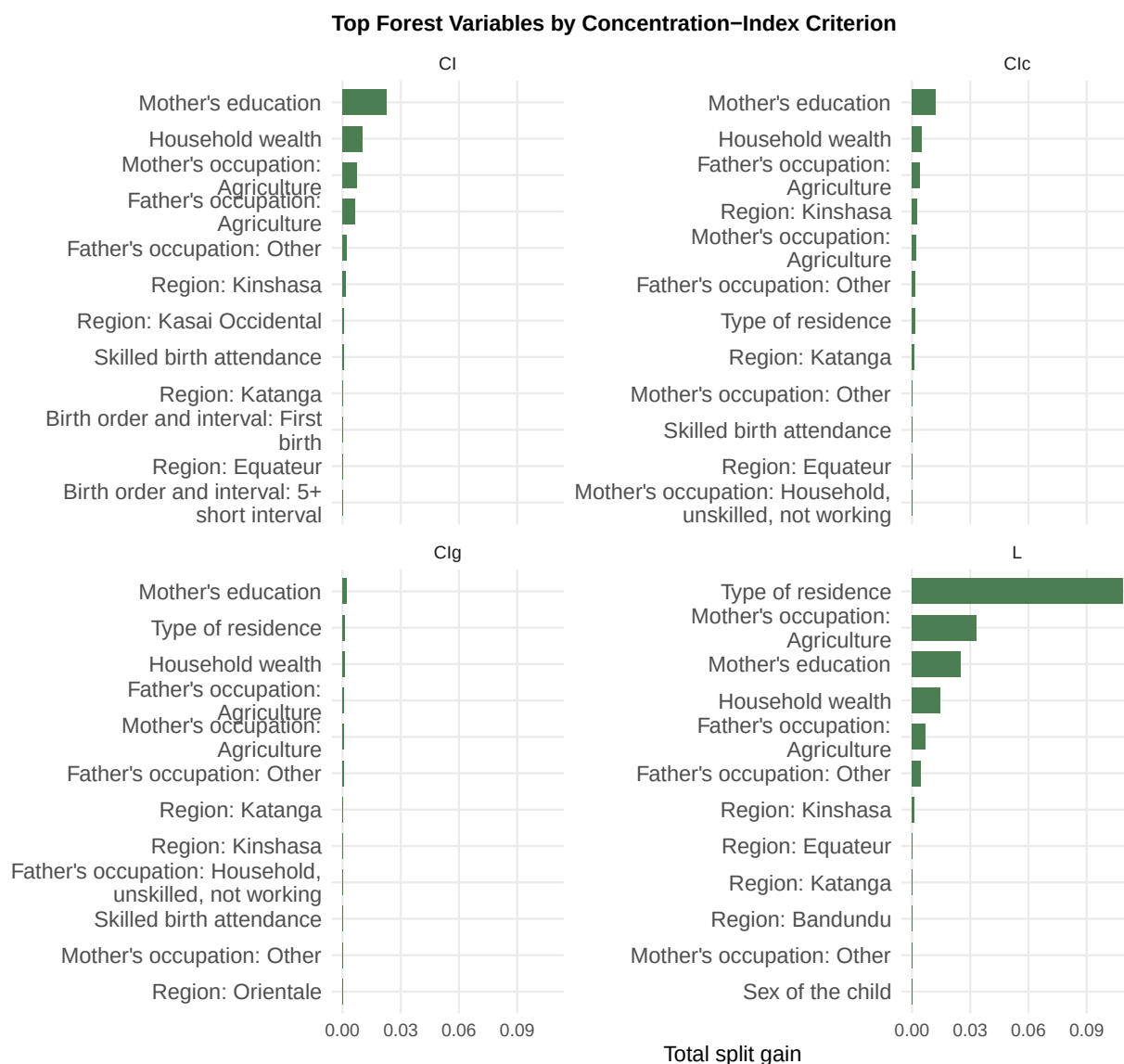
Figure 22: Top forest variables by concentration-index criterion.
