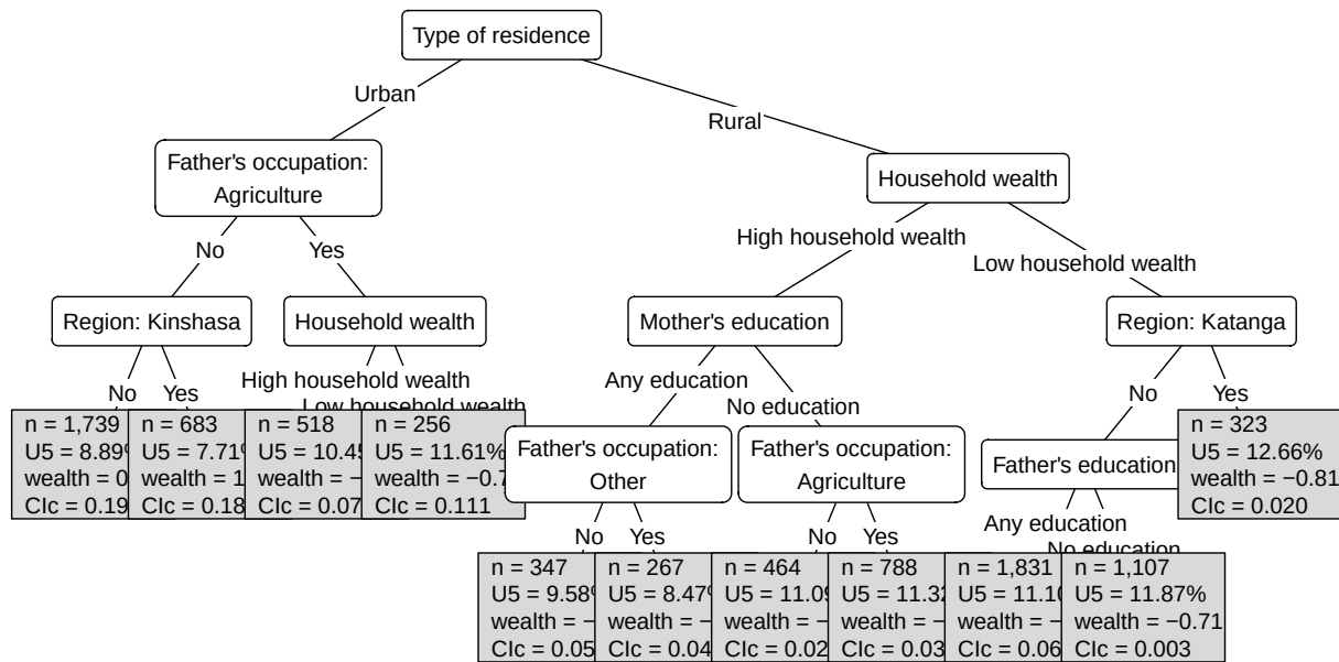
Figure 25: Surrogate tree for the CIc concentration-index forest.
