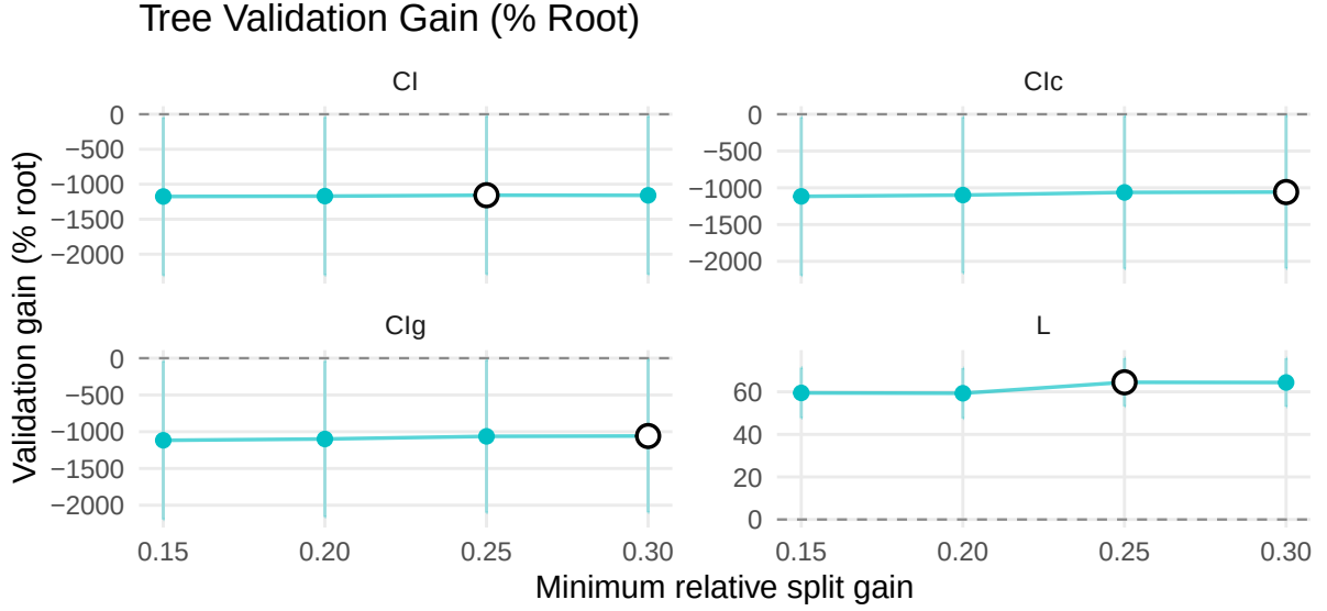
Figure 6: Tree validation gain and complexity by minimum relative split gain.
