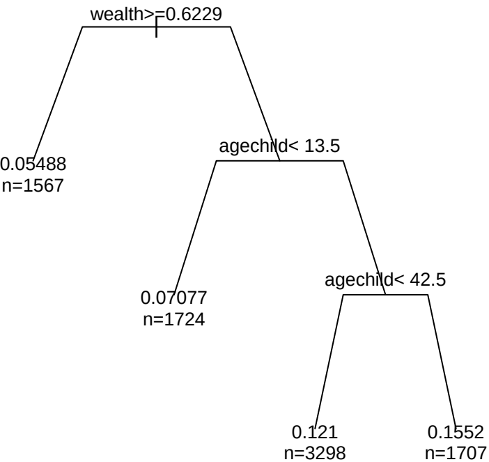
Regression tree (Probability)
