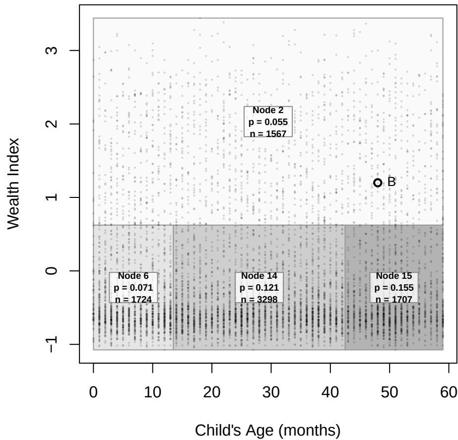
Partition of predictor space
