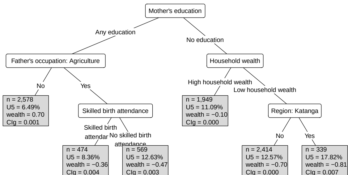
Figure 12: Concentration-index tree fitted with the CIg criterion.
