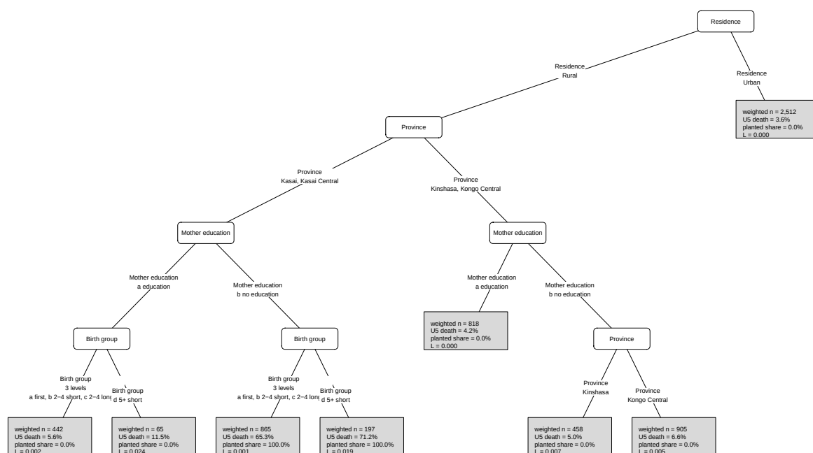
Figure 7: Tree recovered from simulated data with a known subgroup-generating mechanism.
