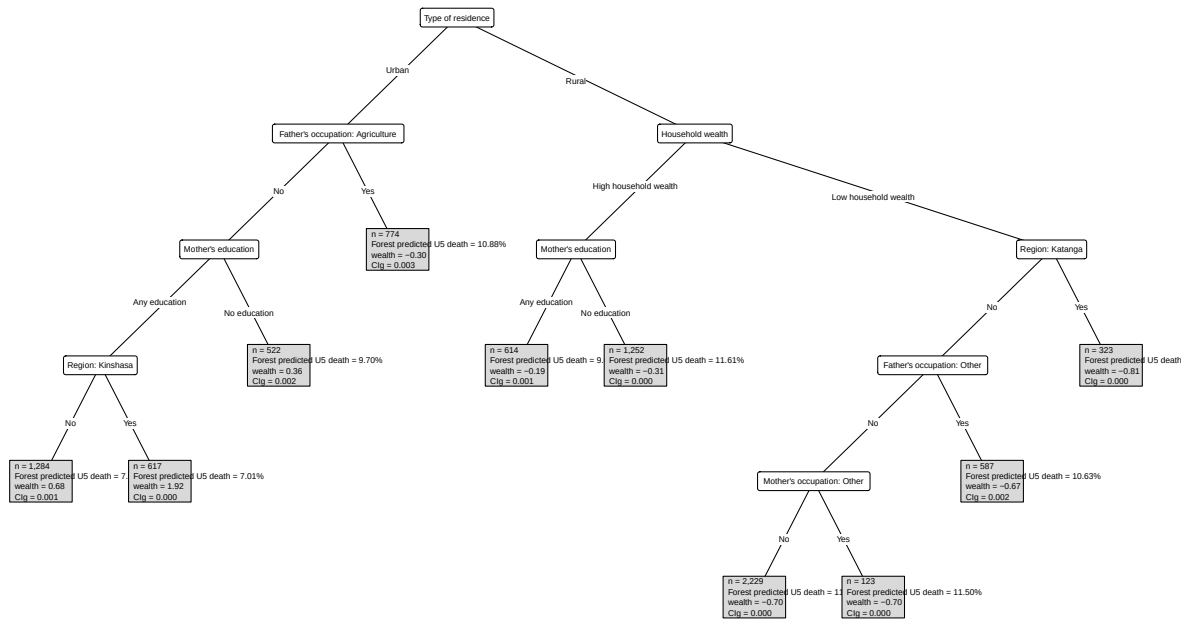
Figure 20: Surrogate tree for the CIg concentration-index forest.
