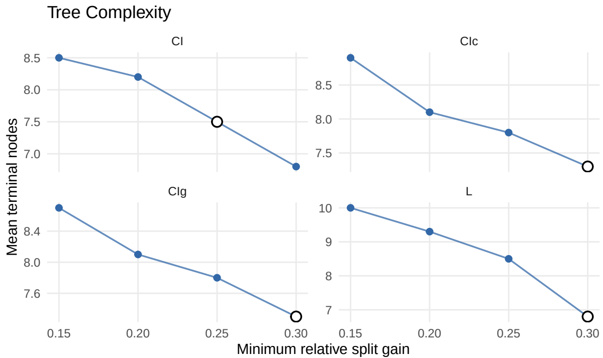
Figure 11: Tree complexity by number of terminal nodes.
