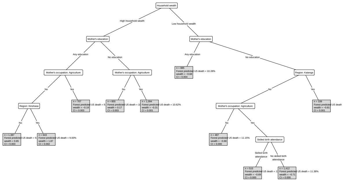
Figure 19: Surrogate tree for the CI concentration-index forest.
