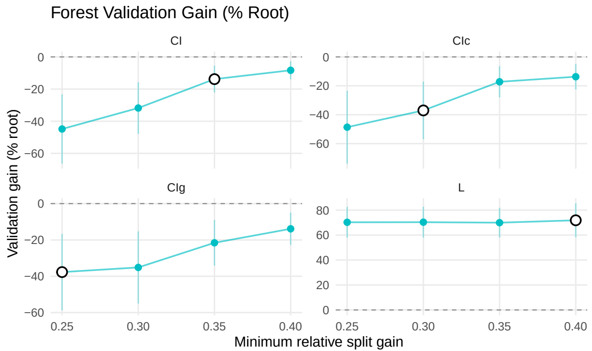
Figure 16: Forest validation gain and complexity by minimum relative split gain.
