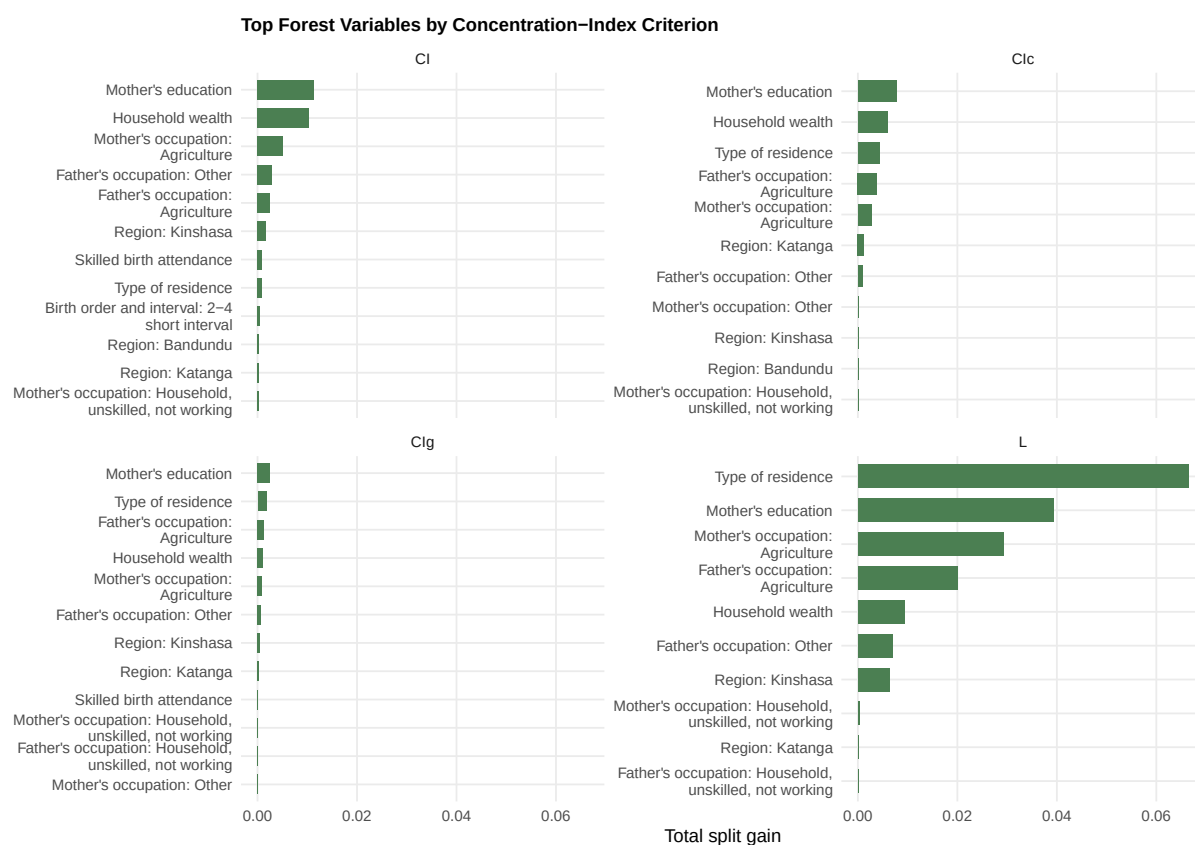
Figure 18: Top forest variables by concentration-index criterion.
