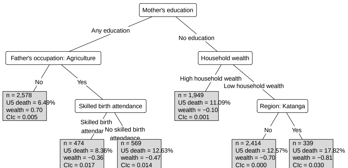
Figure 13: Concentration-index tree fitted with the Clc criterion.
