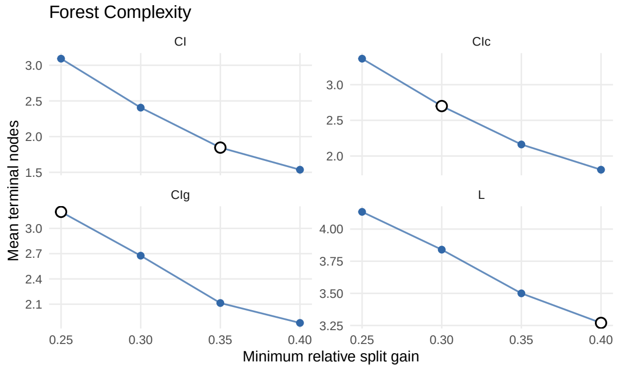
Figure 17: Forest complexity by number of terminal nodes.
