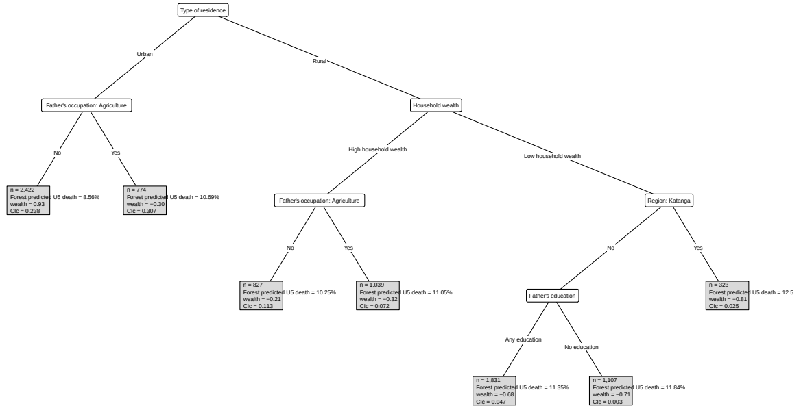
Figure 21: Surrogate tree for the CIc concentration-index forest.
