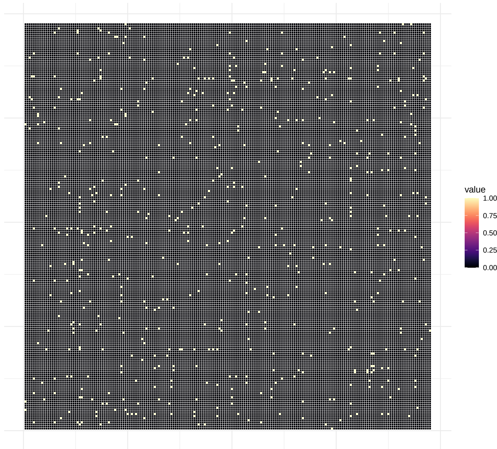
Neighbors
