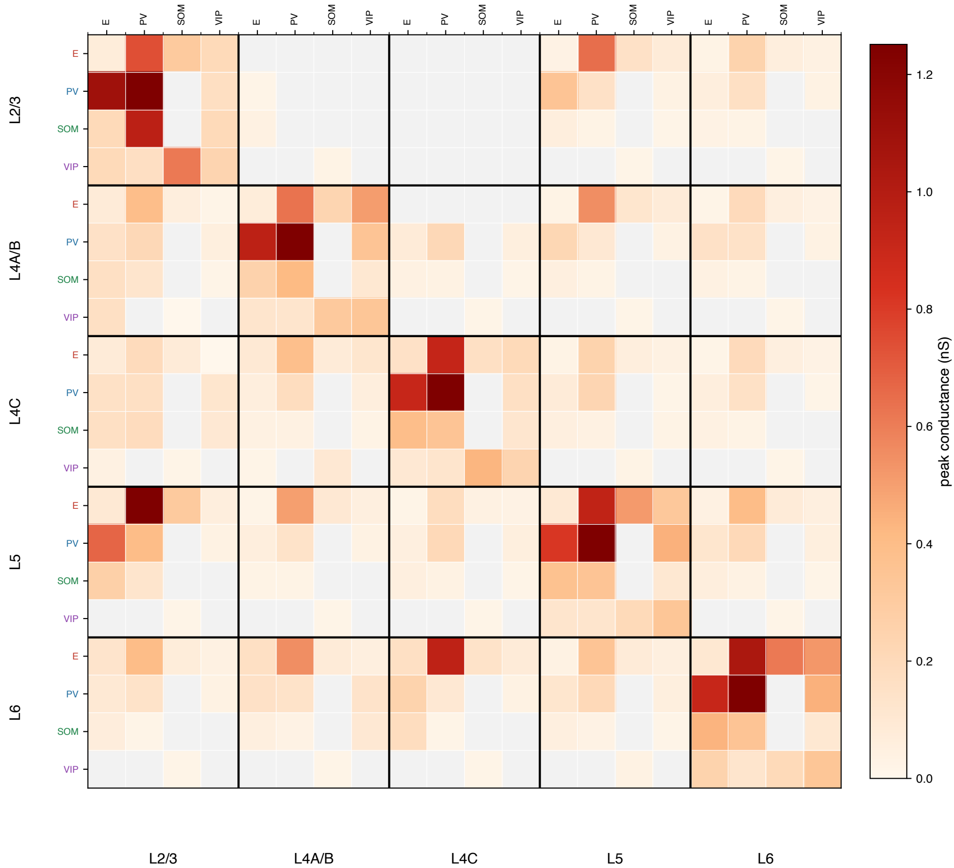
Synaptic weight (AMPA / GABA)
