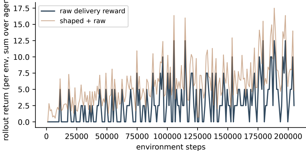
IPPO self-play on overcooked v2 cramped_room (seed 0)
