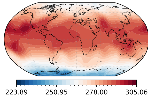
KKR
