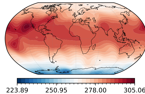
PFNN
