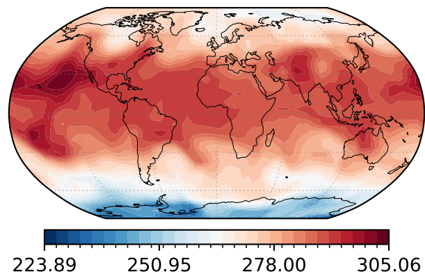
Ground Truth
