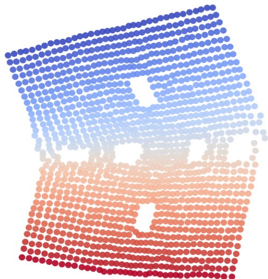
PCC manifold
