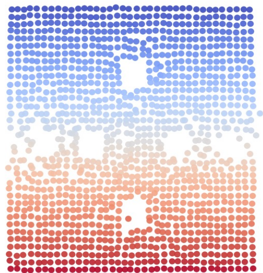
Our manifold
