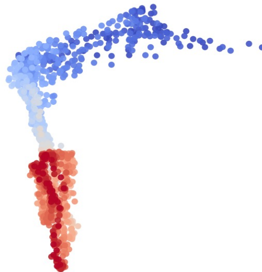
KAE manifold
