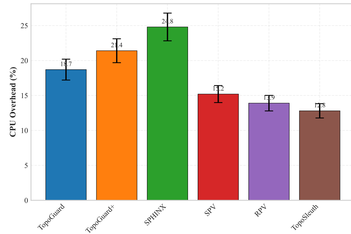
(c) CPU Overhead Comparison
