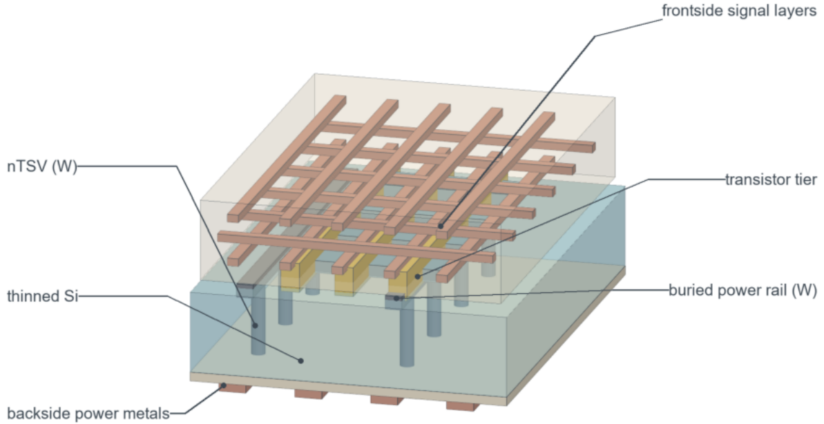
Backside power delivery solid-backend feature testcase
