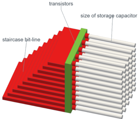
(b) horizontal capacitors, staircase bit-line
