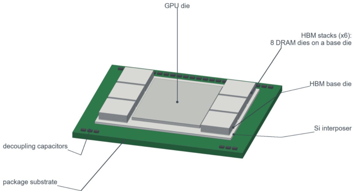
GPU package, CoWoS-style: assembled
