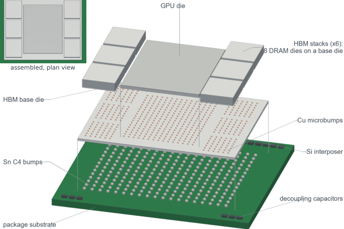
GPU package, CoWoS-style: exploded view
