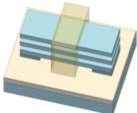
gate-all-around nanosheets
