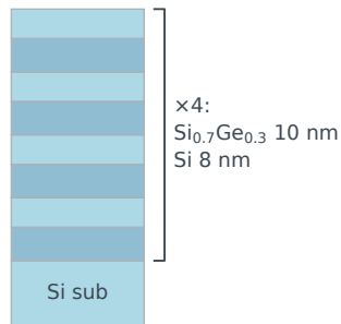
(c) GAA nanosheet stack
