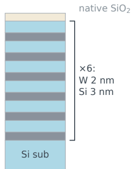
(f) W/Si XRR mirror
