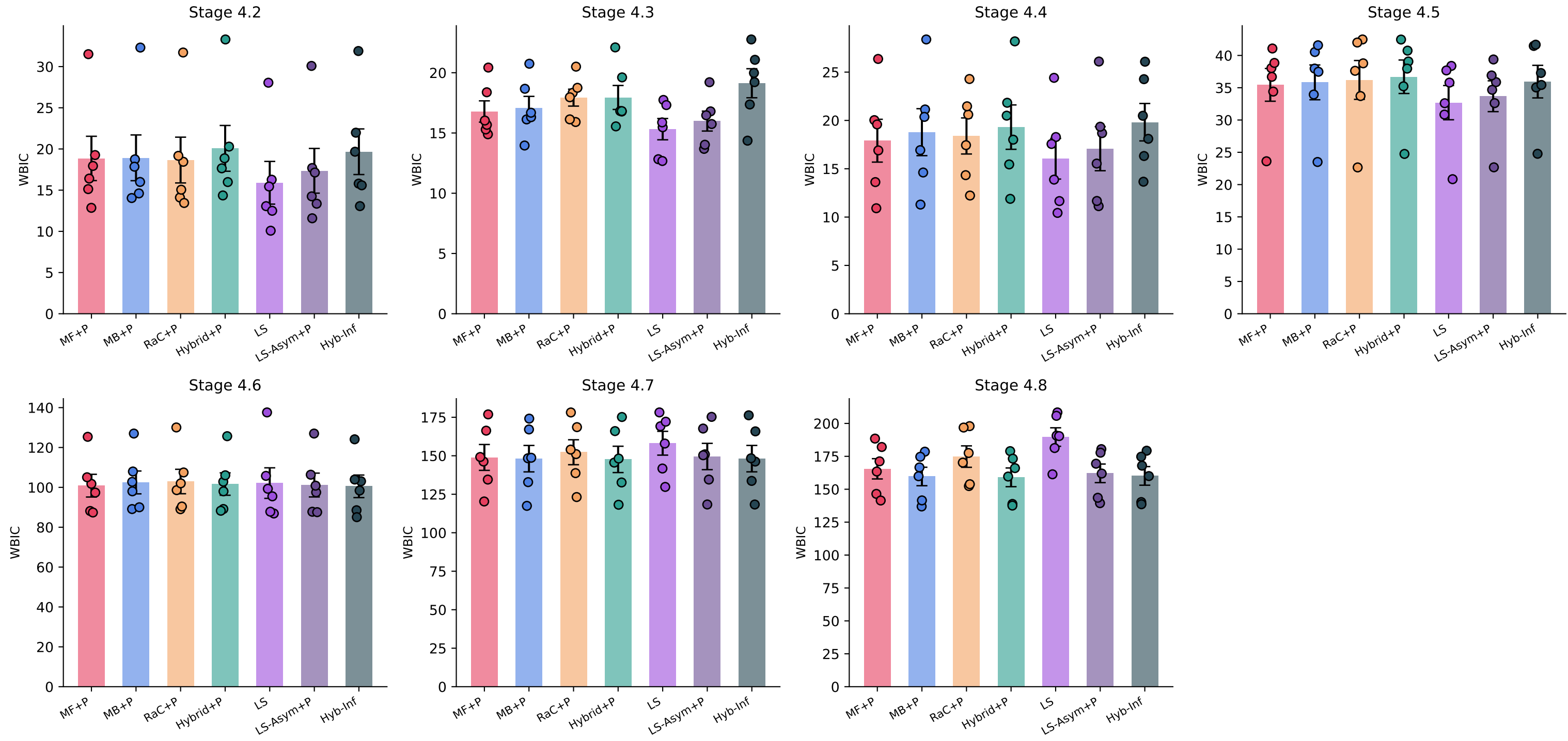
WBIC by Model (lower = better fit)
