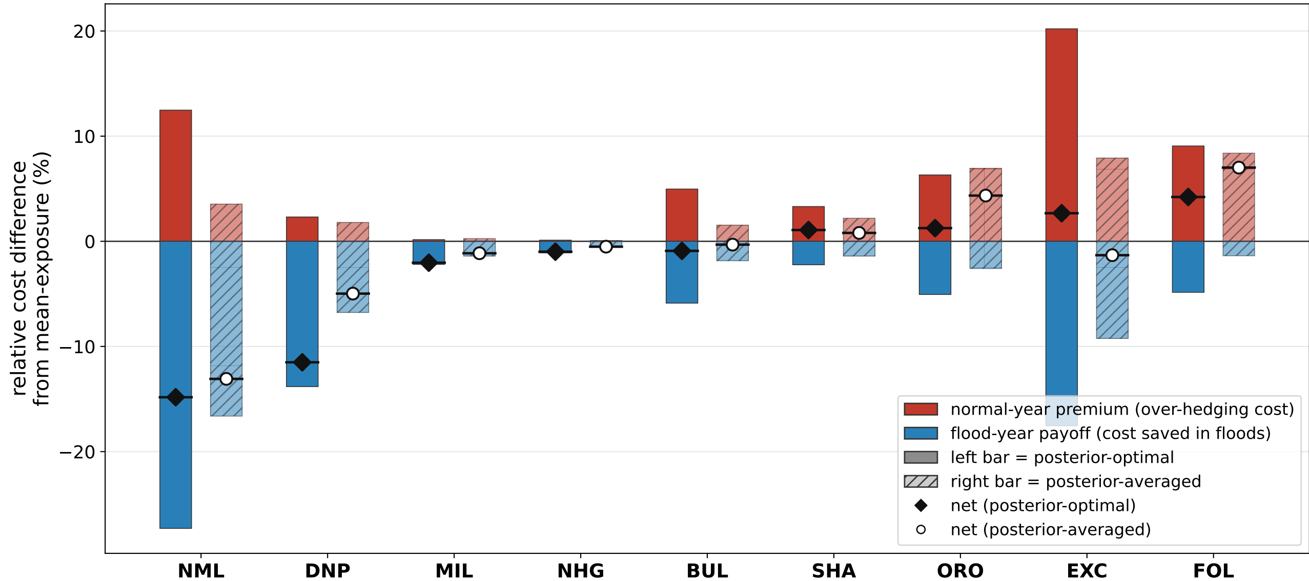
Why the action-selection methods tie on the average: a steady premium offset by rare flood-year payoffs
