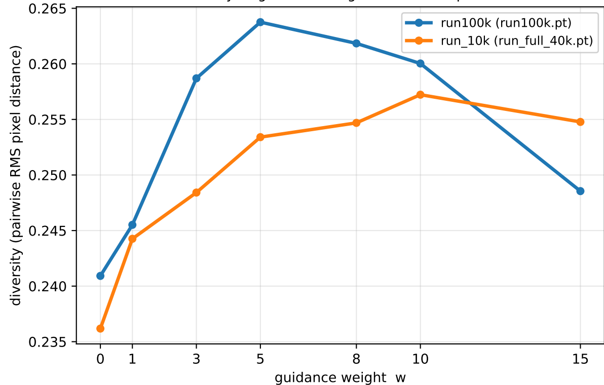
Diversity vs guidance weight — run comparison
