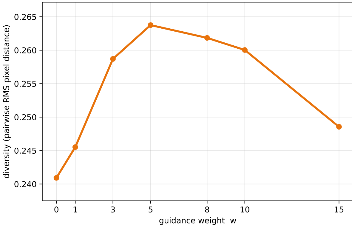
Intra-condition diversity vs guidance weight [run100k] ckpt=run100k.pt, data=10k, sampler=ddpm, conds=16, per cond=8
