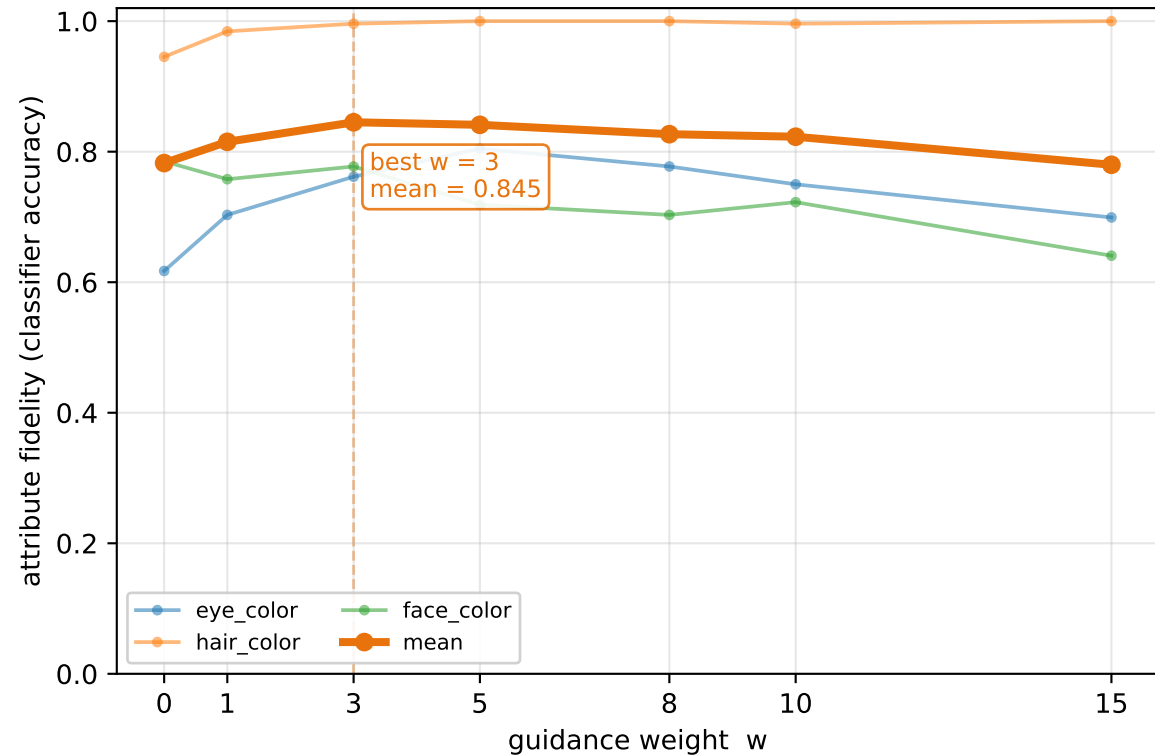
Attribute fidelity vs guidance weight [run_10k] ckpt=run_full_40k.pt, data=10k, sampler=ddpm, n=256
