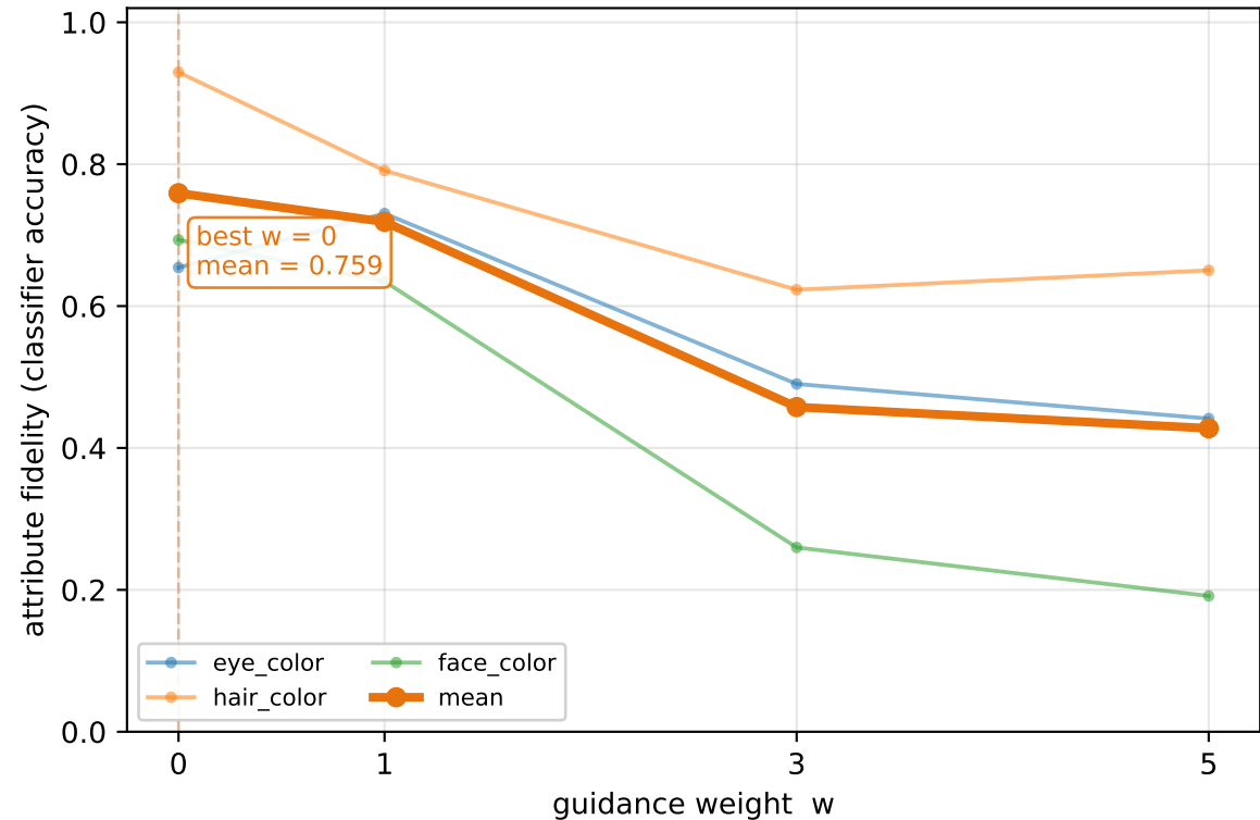
Attribute fidelity vs guidance weight [run_full_40k_ddim, 10k, n=512, 50 DDIM steps]
