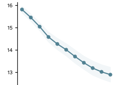
adjusted weights
