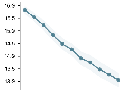
random weights
