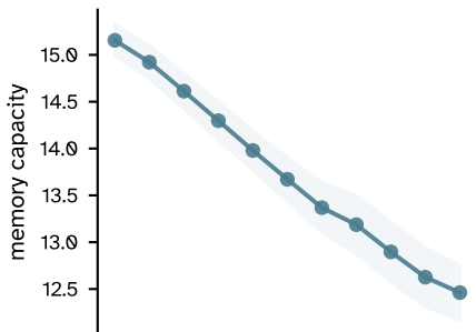
binary
