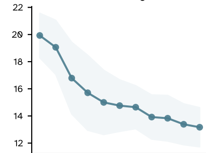
random weights
