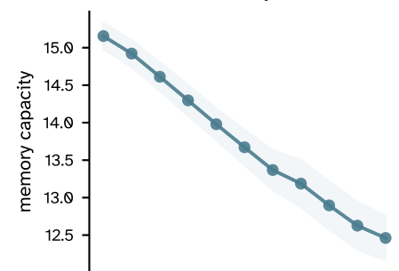
binary
