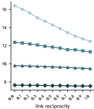
memory capacity
