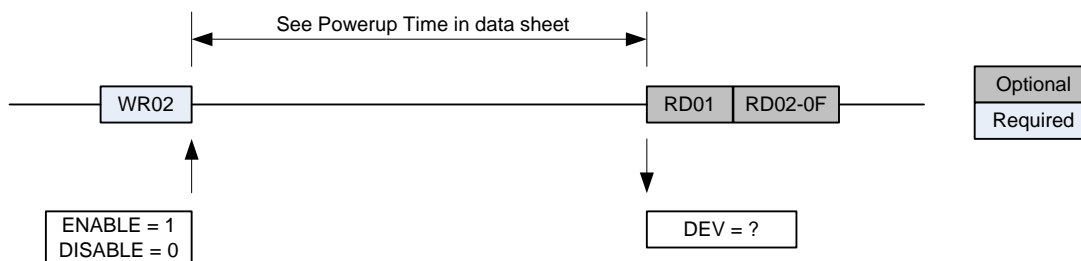
Figure 8. Powerup Timing
