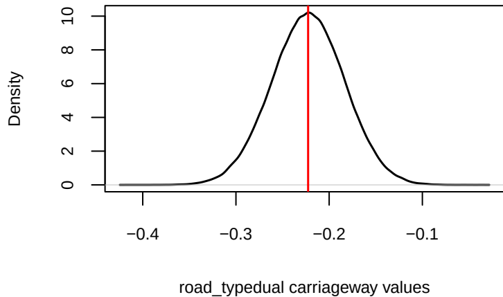
CMC posterior density of road_typedual carriageway
