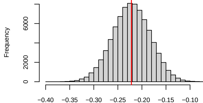
Posterior histogram of road_typedual carriageway
