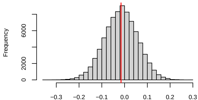
Posterior histogram of road_typeone way street (from 2005)
