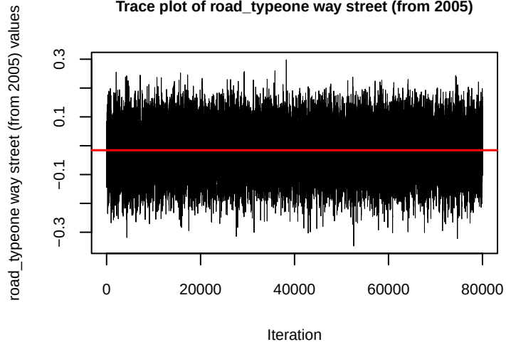
Trace plot of road_typeone way street (from 2005)
