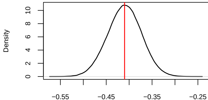
CMC posterior density of road_typeroundabout
