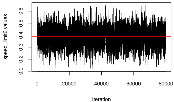
Trace plot of speed_limit6
