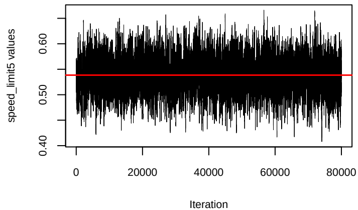
Trace plot of speed_limit5
