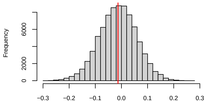
Posterior histogram of road_typeone way street (from 2005)
