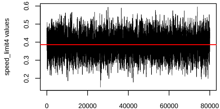
Trace plot of speed_limit4
