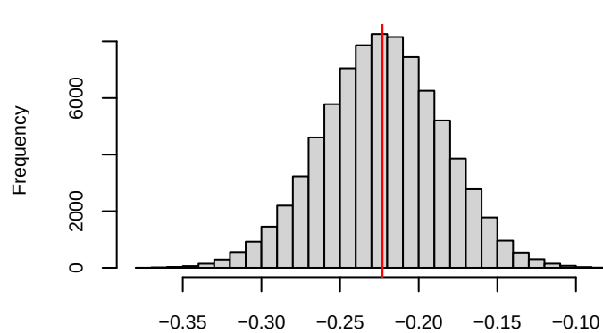
Posterior histogram of road_typedual carriageway
