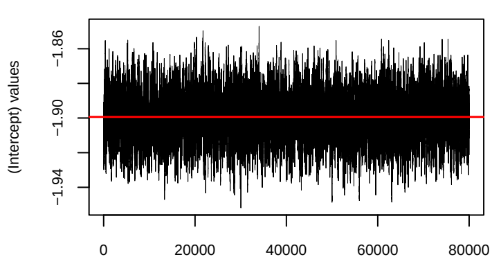
Trace plot of (Intercept)
