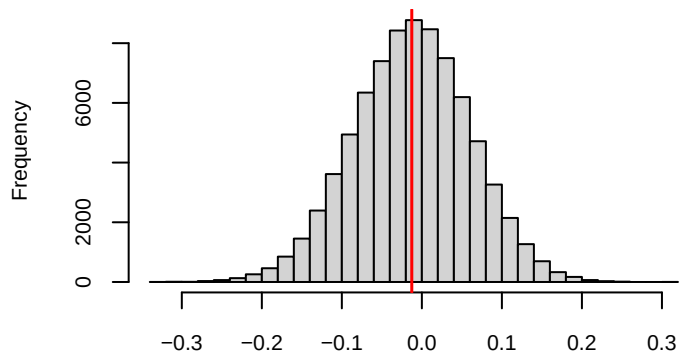
Posterior histogram of road_typeone way street (from 2005)
