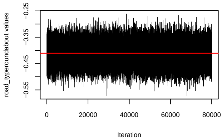
Trace plot of road_typeroundabout
