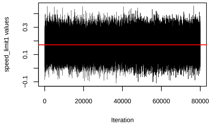
Trace plot of speed_limit1
