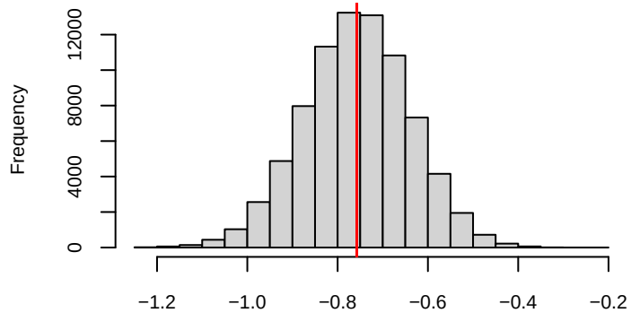
Posterior histogram of road_typeslip road (from 2005)
