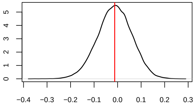
CMC posterior density of road_typeone way street (from 2005)
