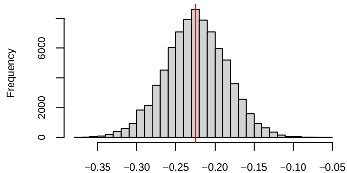
Posterior histogram of road_typedual carriageway
