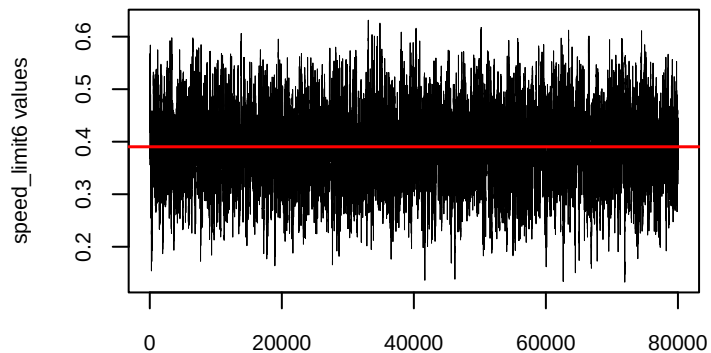
Trace plot of speed_limit6
