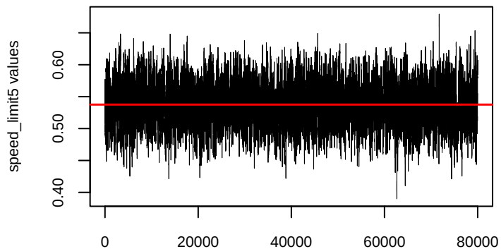
Trace plot of speed_limit5
