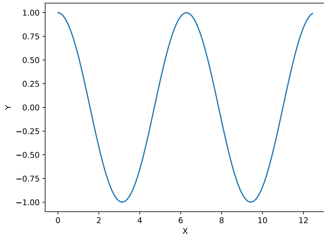
Cosine Wave
