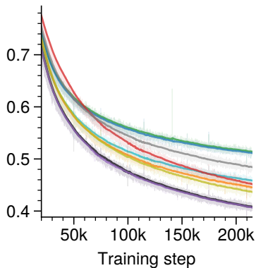
F-IID Policy
