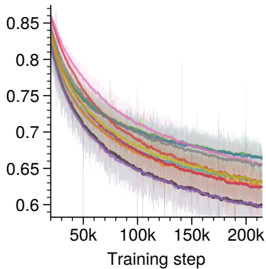
Patch MSE
