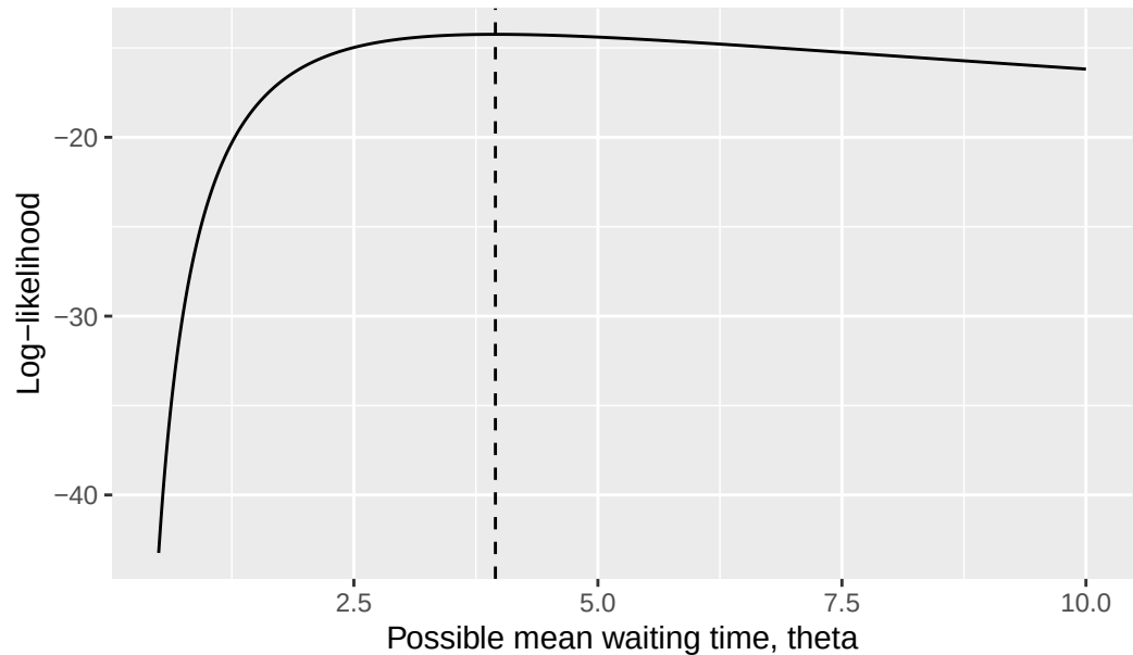
Log-likelihood for the exponential waiting-time model
